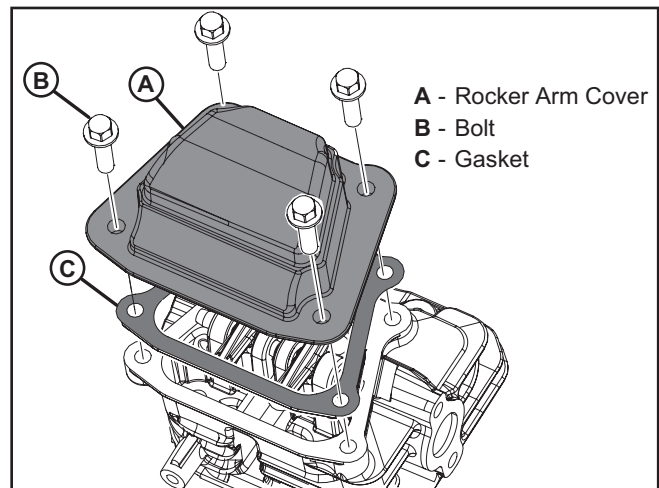
Figure 40 – Removing the Rocker Arm Cover
