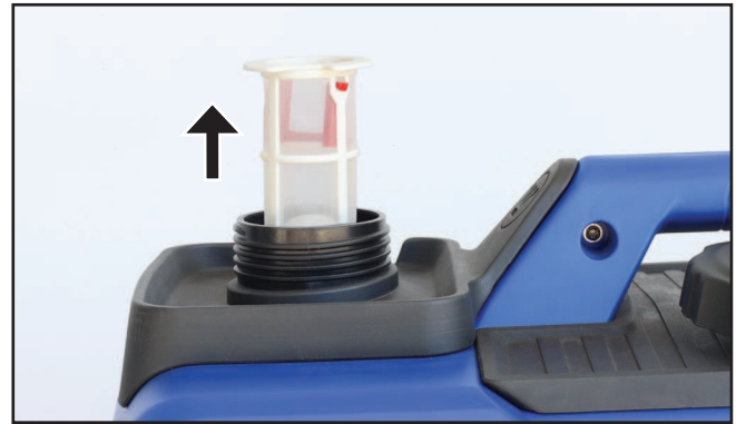
Figure 30 – Removing the Fuel Strainer
