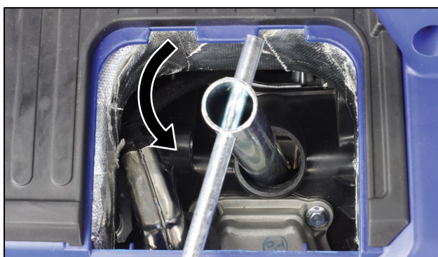
Figure 40 Remove the Spark Plug
