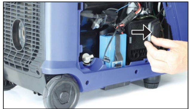
Figure 30 Remove the Air Filter Cover
