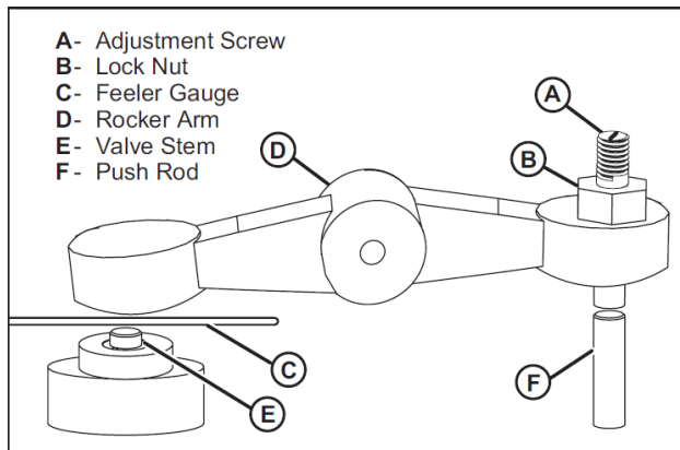
Figure 45 Set Valve Clearance
