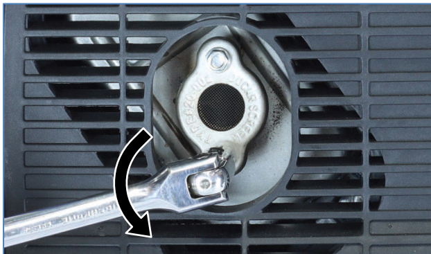
Figure 42 Remove the Spark Arrestor Clamp
