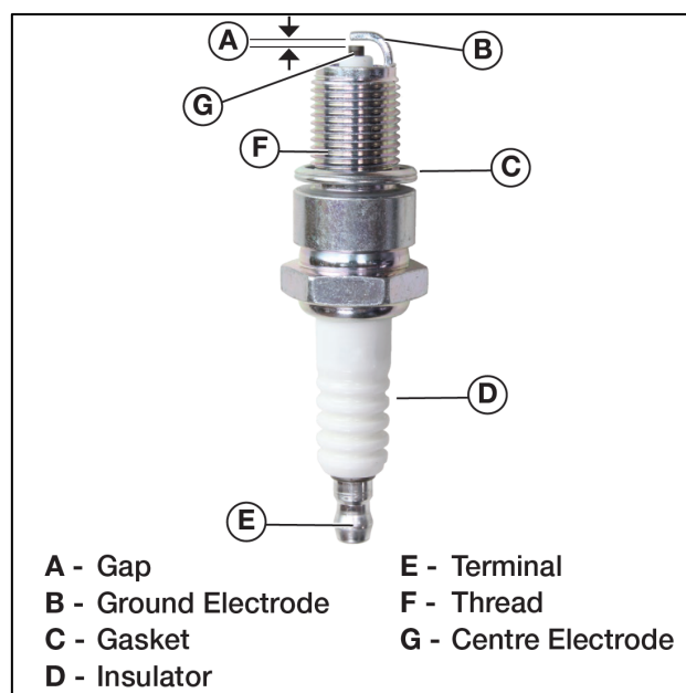
Figure 41 Spark Plug
