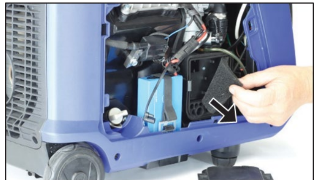
Figure 31 Remove the Air Filter Element
