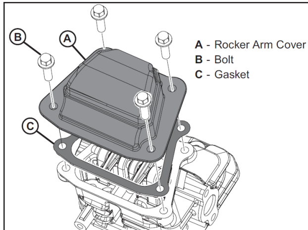
Figure 44 Access for Valve Clearance
