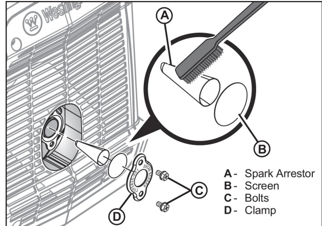
Figure 43 Remove and Clean the Spark Arrestor
