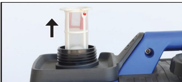
Figure 32 Remove the Fuel Strainer
