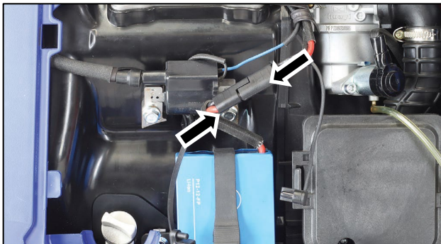
Figure 6 Assemble the Battery Wiring Harness Connector
