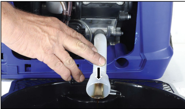
Figure 20 Drain the Engine Oil
