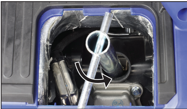
Figure 24 – Removing the Spark Plug
