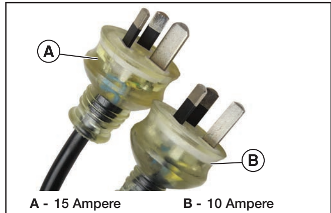
Figure 22 – 240-Volt AC Three-Pin Plugs
