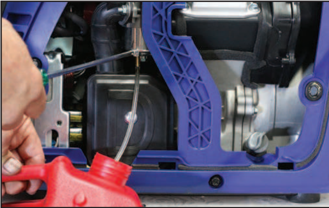
Figure 52 – iGen2200 & 2500 Draining the Carburettor
