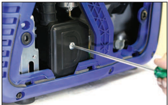
Figure 36 - iGen2200 & 2500 Removing the Air Filter Cover
