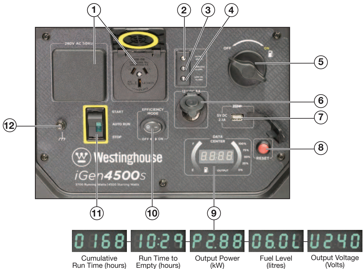
Figure 8 - iGen4500s Control Panel Features
