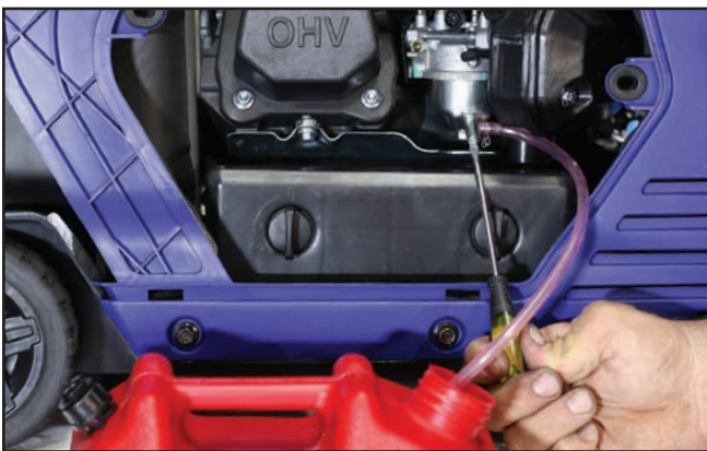
Figure 53 – iGen4500s Draining the Carburettor
