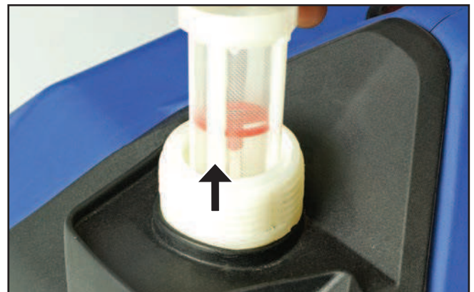
Figure 39 – Removing the Fuel Strainer
