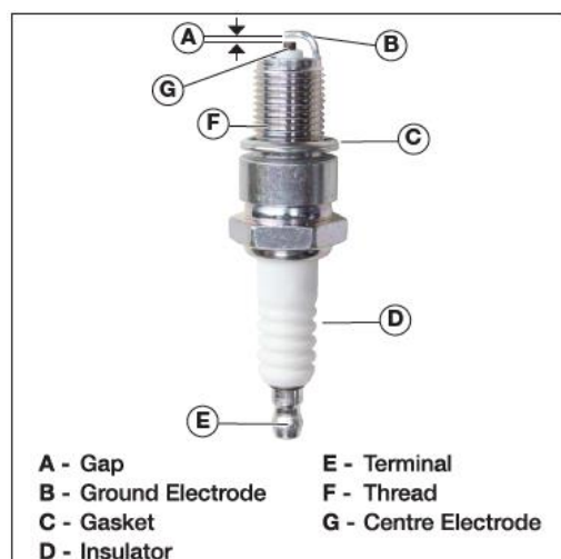
Figure 45 Spark Plug
