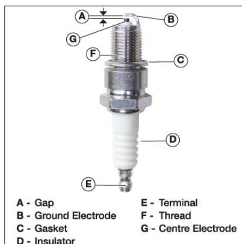
Figure 45 Spark Plug
