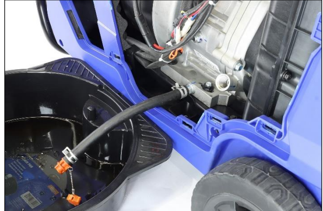
Figure 33 Draining the Engine Oil
