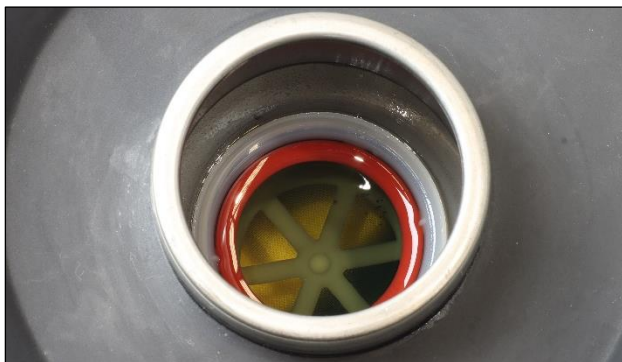
Figure 12 Maximum Fuel Fill Level
