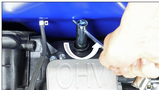
Figure 44 Remove the Spark Plug
