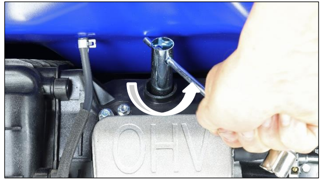
Figure 44 Remove the Spark Plug
