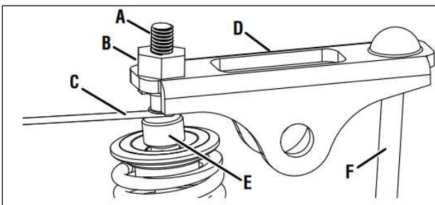
A – Adjustment Screw D – Rocker Arm B – Lock Nut E – Valve Stem C – Feeler Gauge F – Push Rod
