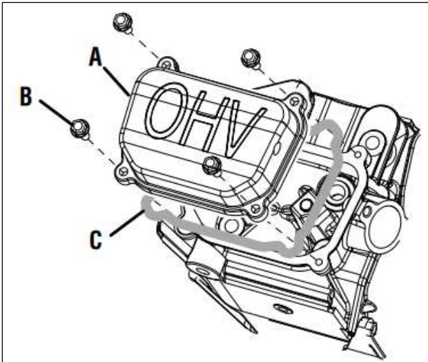
A – Rocker Arm Cover C – Gasket B – Bolt
