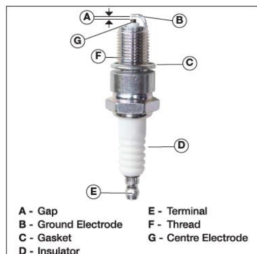
Figure 45 Spark Plug
