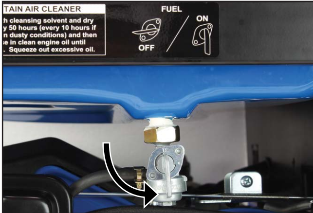
Figure 16 – Fuel Shutoff Valve in the ON Position
