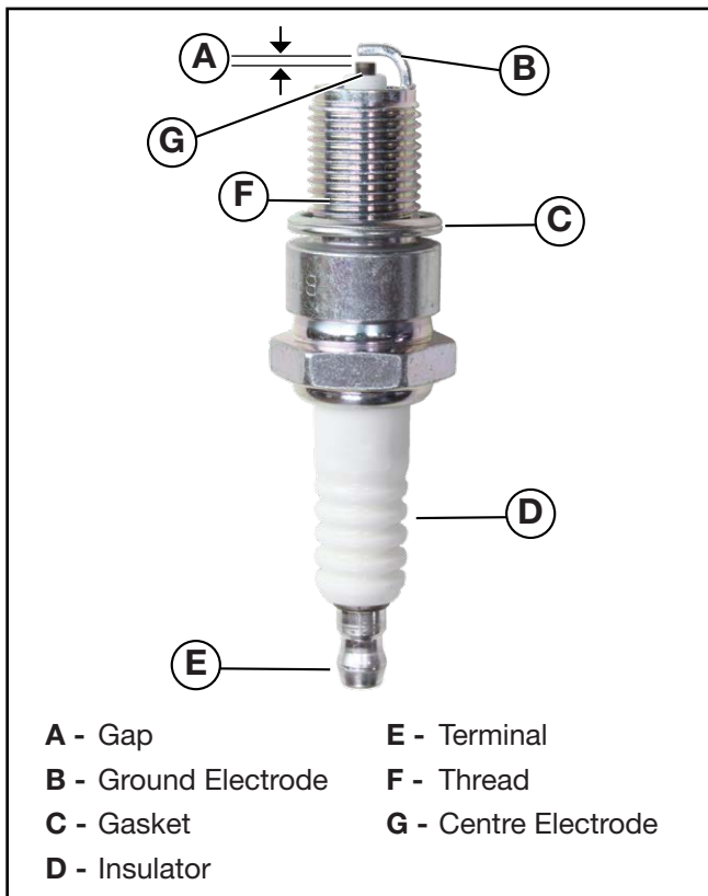
Figure 49 – Spark Plug
