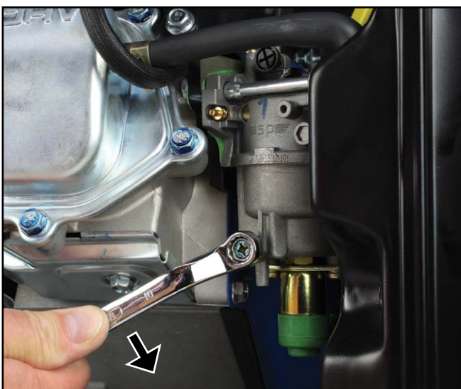
Figure 57 – Removing the Carburettor Drain Screw (WHXC5000, WHXC7000, WHXC8500E, WHXC8500E-PRO & WHXC8500E-AS)
